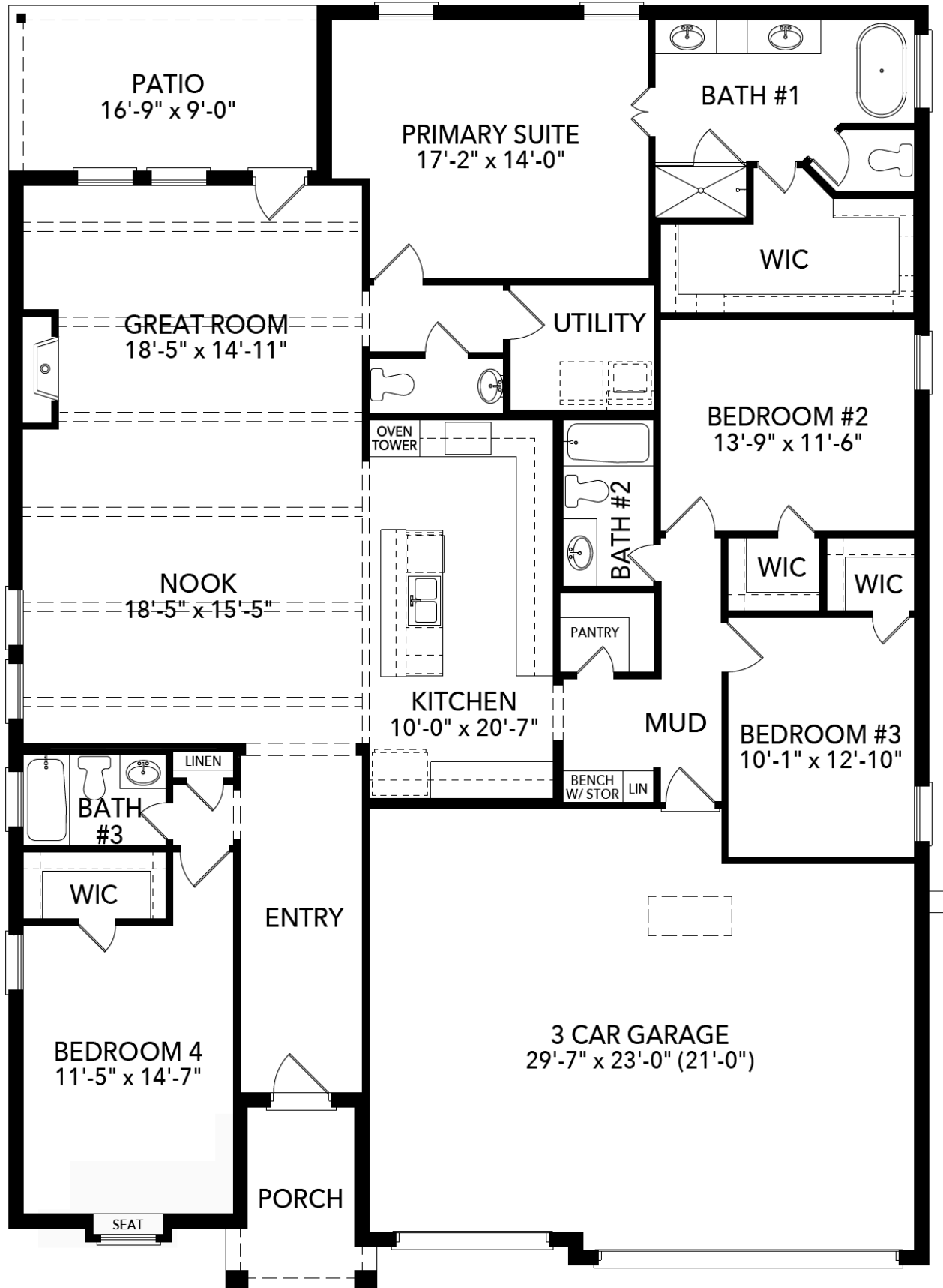
First Floor
